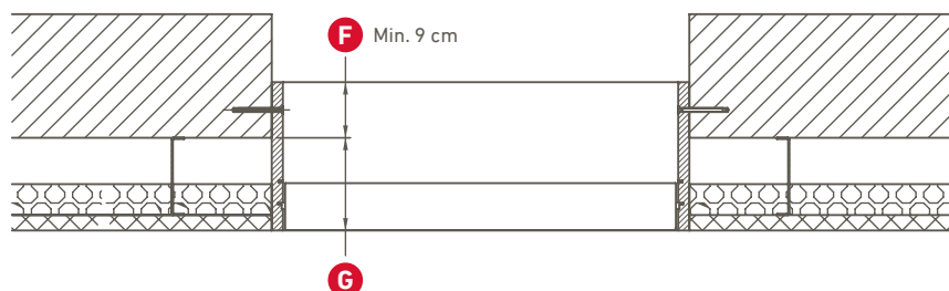
Suspended ceiling
